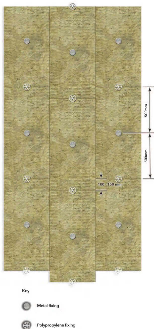
Figure 4: Typical fixing pattern with 3 fixings per square metre
