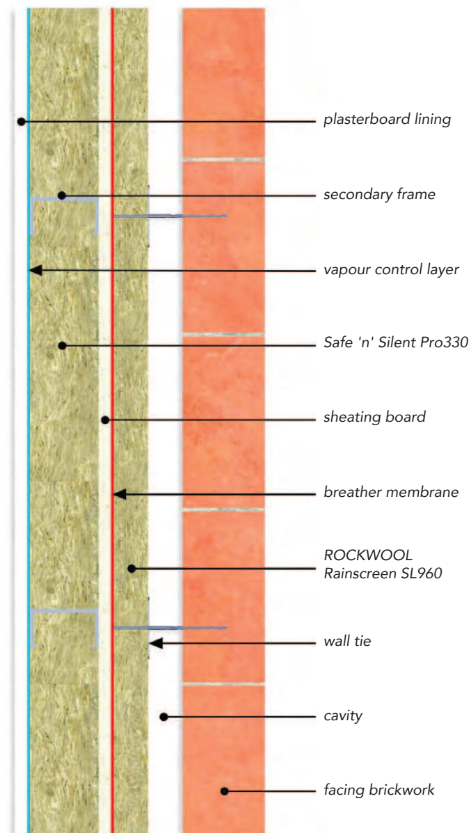
Figure 3: ROCKWOOL Rainscreen insulation for cladding systems with masonry outer leaf
