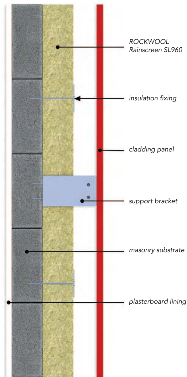
Figure 2: ROCKWOOL Rainscreen insulation for cladding systems with concrete/masonry
